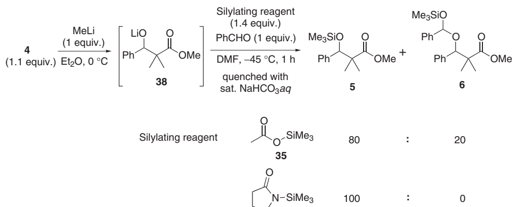
Scheme 7. Silylation of lithium aldolate 38 in the co-existence of benzaldehyde.
