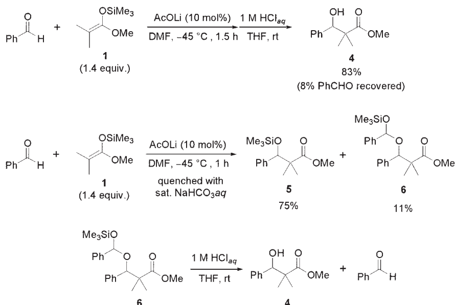
Scheme 4. AcOLi-catalyzed aldol reaction between TMS enolate 1 and benzaldehyde in DMF.
