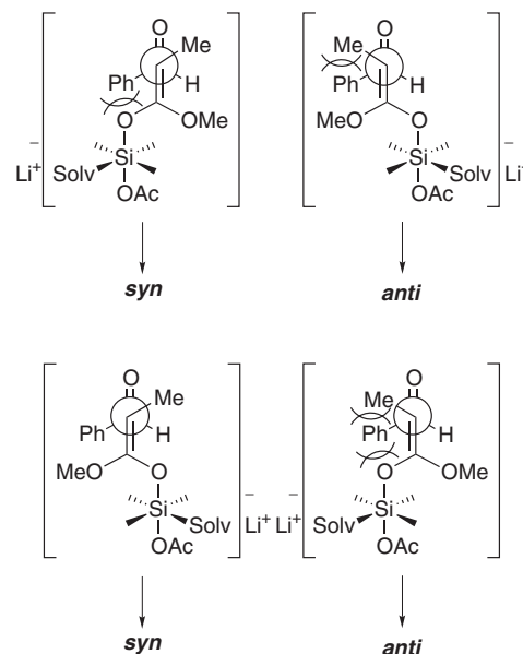
Fig. 1. Difference of reactivity between E - and Z -enolate.
