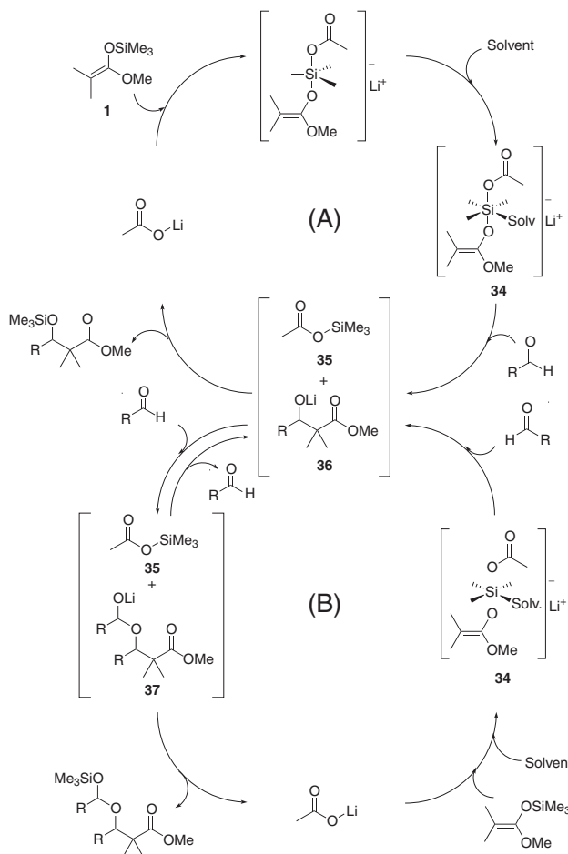
Scheme 6. Assumed catalytic cycle of AcOLi-catalyzed aldol reaction in anhydrous DMF or pyridine.
