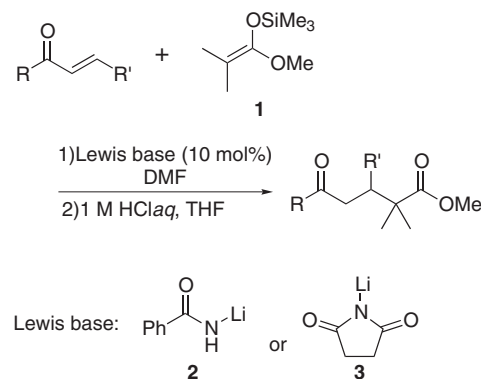
Scheme 2. Lewis base-catalyzed Michael reaction between ketene silyl acetals and \alpha,\beta -unsaturated carbonyl compounds.
