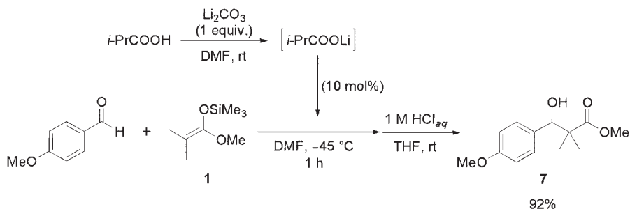
Scheme 5. Aldol reaction by using i -PrCOOLi prepared from i -PrCOOH and lithium carbonate.
