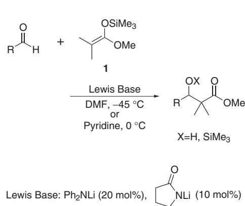
Scheme 1. Lewis base-catalyzed aldol reaction between aldehyde and trimethylsilyl enolate.
