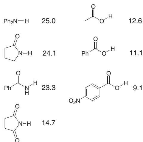
Scheme 3. pK_a values of acidic hydrogens in dimethyl sulfoxide.
